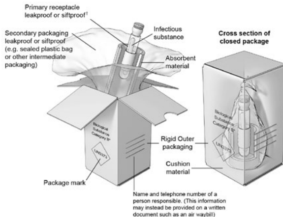
Figure 2. A Category B Non-specification Triple Packaging
